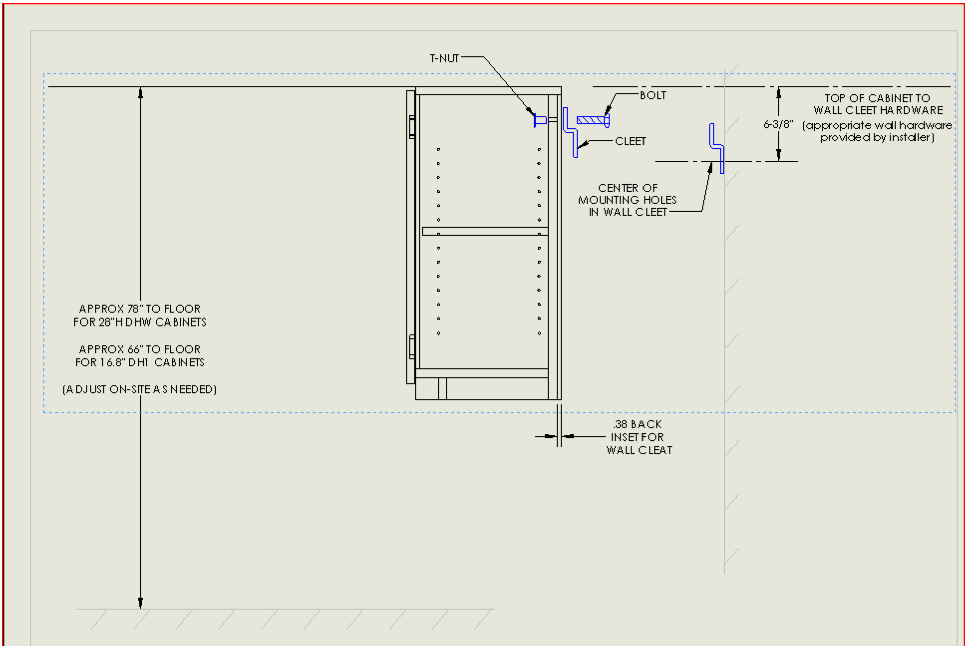
AFFINITY OVERHEAD WALL-MOUNT CABINETS INSTALLATION INSTRUCTIONS
